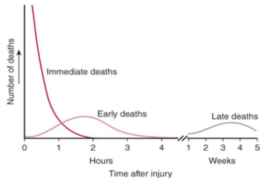
Figure 3: Literature reports the advanced evolution of mortality for shock.
