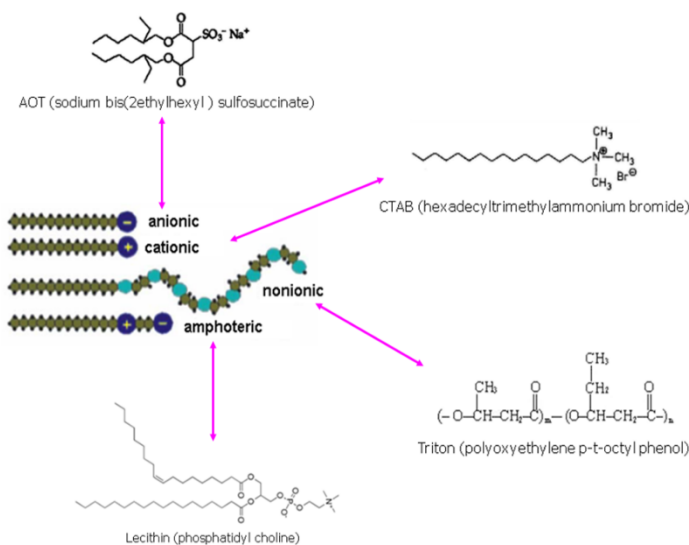
Figure 2: Examples of surfactants belonging to different types.
