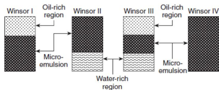
Figure 3: Winsor classification system, showing oil- and water-rich phases possible in microemulsion systems. Redrawn with permission.20 Copyright (1997) C.R.C. Press.13
